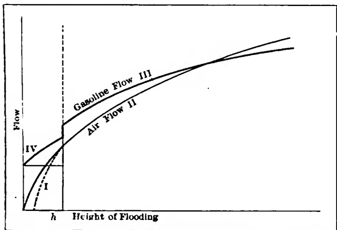
Fig. 6—Curves taken from tests of the Vapor carburetor, the dotted line I indicating the flow of gasoline up to the time the well floods
